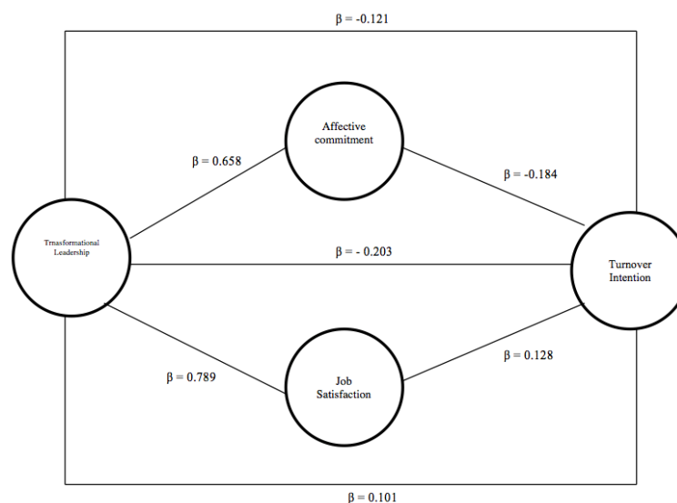
Figure 3. Structural equation modeling (SEM)
