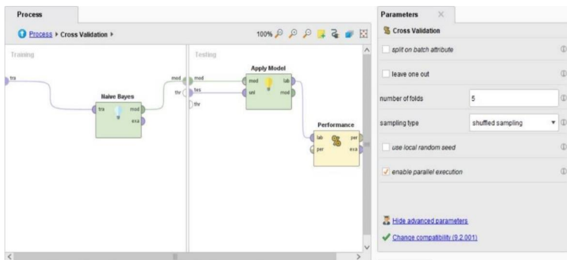
Figure 3. Cross-Validation Process
