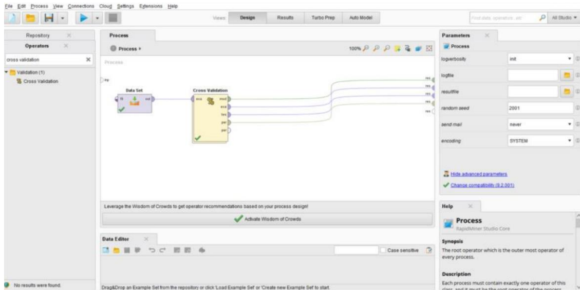
Figure 2. Cross-Validation Connection
