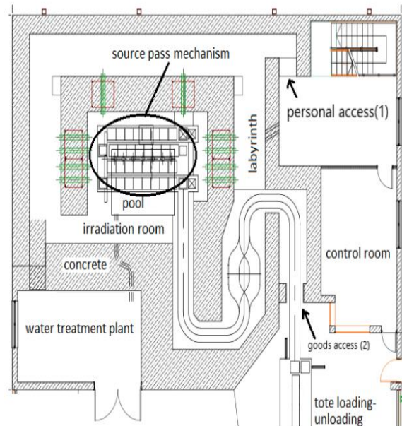
Fig. 1. Working principle of Irradiator [6]
