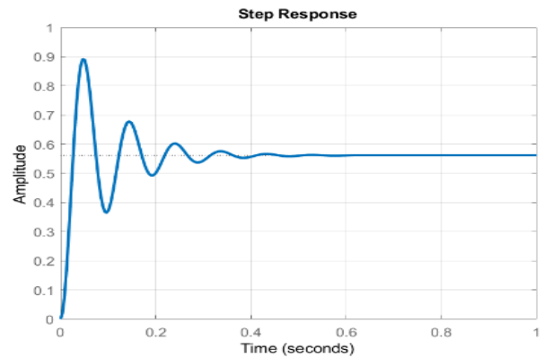
Fig. 3. Transient response of G_m system without a controller
