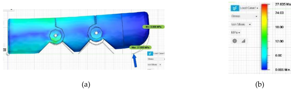
Figure 10. (a) (b) Stress Analysis Results
