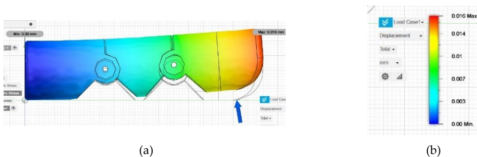
Figure 9. (a) (b) Deformation Analysis Results
