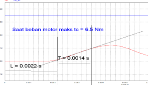
Fig 10. Simulation results with a torque load of 6.5 Nm
