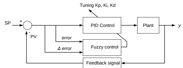
Fig. 4. Autotuning PID Fuzzy Control
