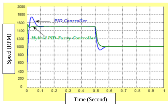
Fig. 23. Speed 1500 rpm to 1000 rpm with load.
