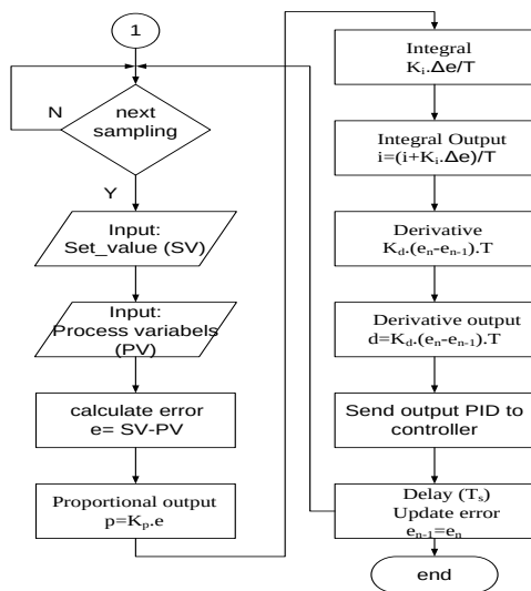
Fig 12. Flowchart Autotuning PID Fuzzy Controller
