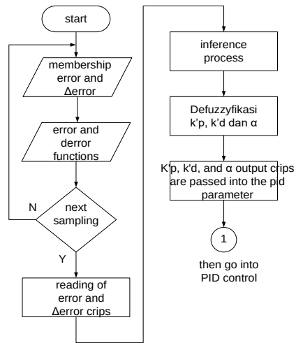
Fig 11. Flow chart reading of k'_p , k'_d , and \alpha values
