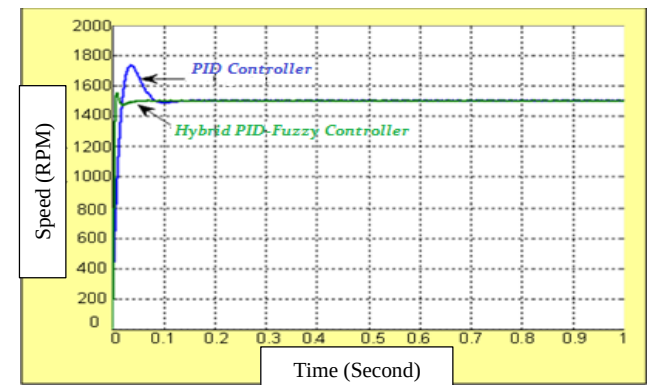
Fig. 19. Speed to 1500 rpm set point with load
