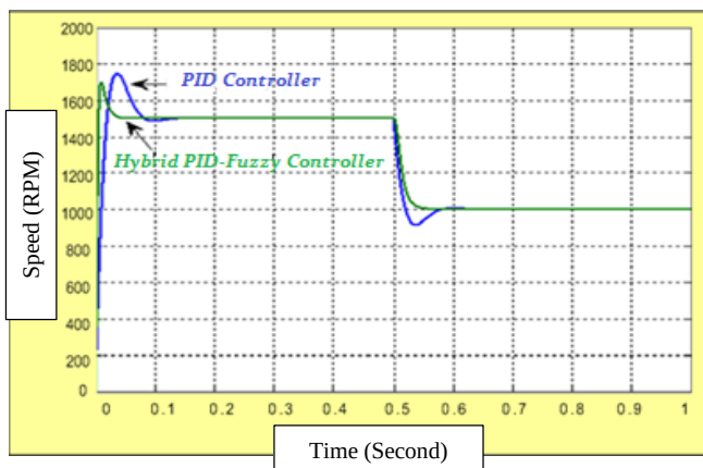
Fig. 22. Speed 1500 rpm to 1000 rpm no load
