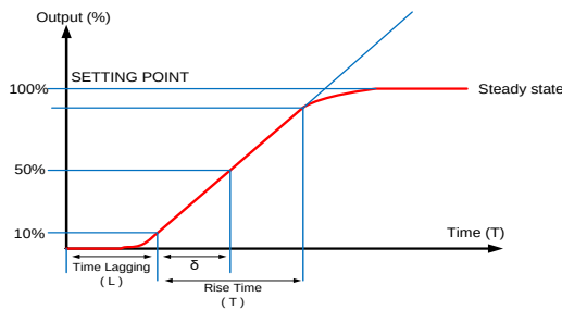
Fig. 2. The reaction process curve
