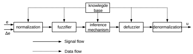
Fig 5. Fuzzy logic controller
