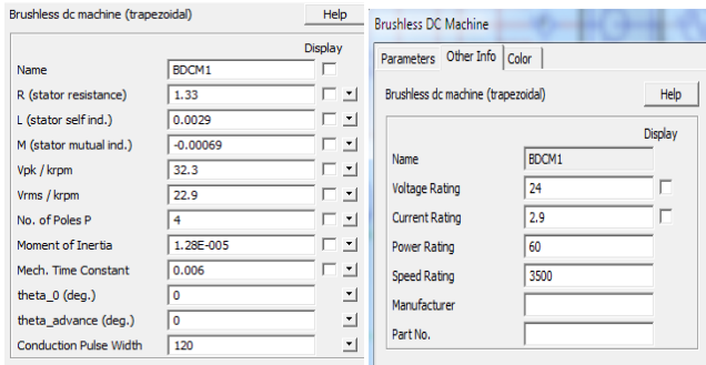
Fig 7. BLDC Motor specification
