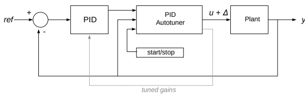
Fig. 3. PID Autotuning control
