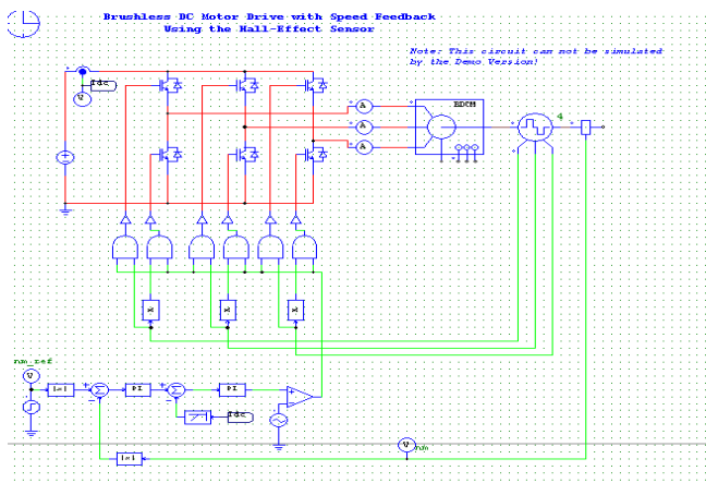
Fig 8. Circuit simulation experiment with BLDC motors using the program PSIM
