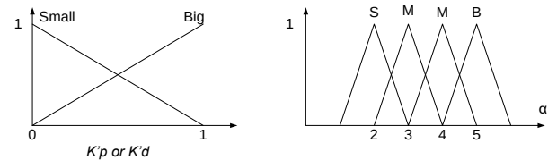
Fig 16. Membership functions k'_p , k'_d and \alpha
