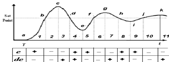
Fig 14. Step system response
