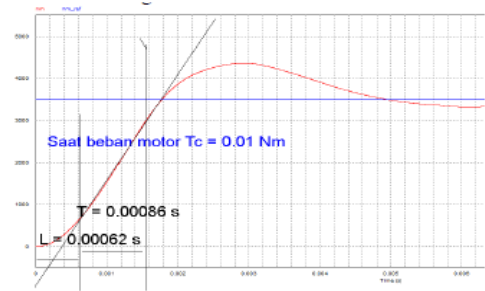
Fig 9. Simulation results with a torque load of 0.01 Nm
