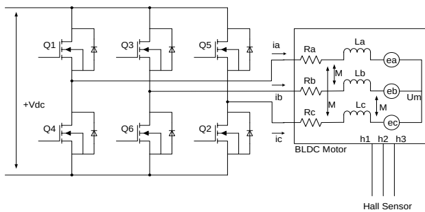
Fig 1. Motor drive and ekuivalen BLDC Motor
