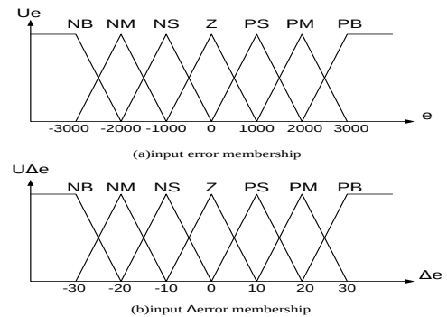
Fig 15. Membership of error and \Delta error
