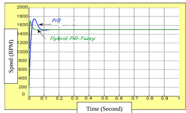
Fig. 18. Speed to 1500 rpm set point no load
