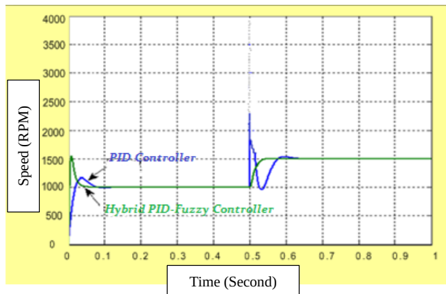
Fig. 21. Speed 1000 rpm to 1500 rpm with load
