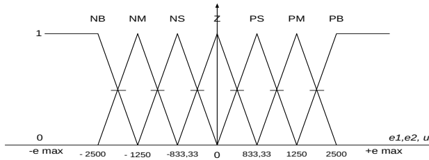
Fig 6. Membership function for e and \Delta e .
