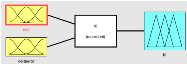
Fig. 8. Block fuzzy for Ki output
