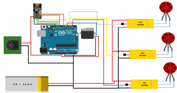
Fig. 11. Circuit diagram of the receiver circuit.
