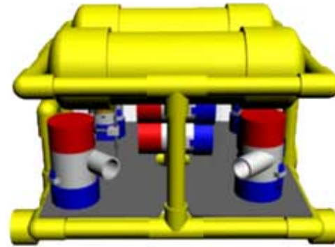
Fig. 5. Side view design in AutoCAD.
