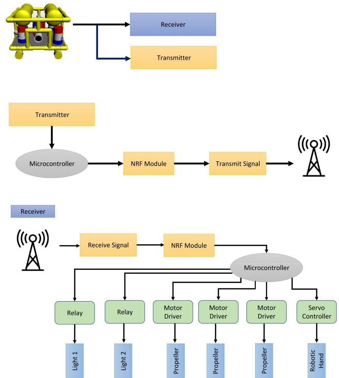
Fig. 1. Block diagram of the proposed underwater drone.
