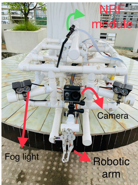
Fig. 6. Front view of the proposed underwater drone.
