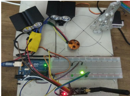
Fig. 10. Receiver circuit of the proposed system.
