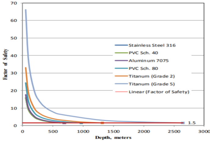
Fig. 2. Different materials factor of safety vs. depth in meter graph.
