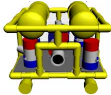
Fig. 4. Front view design in AutoCAD.
