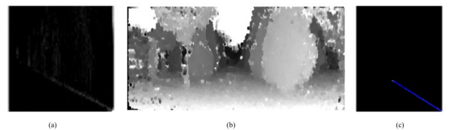
Fig. 14. Converting the disparity map in to v disparity image (a) and detecting the line that would represent the road surface (c) from the refined disparity map (b)
