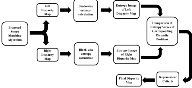
Fig. 7. Diagrammatic representation of ESR methodology for disparity map refinement
