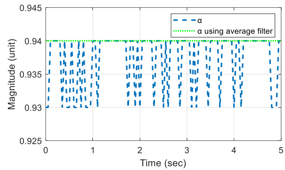
Fig. 18. The results of \alpha in relation to joystick was held in place for 5 sec.
