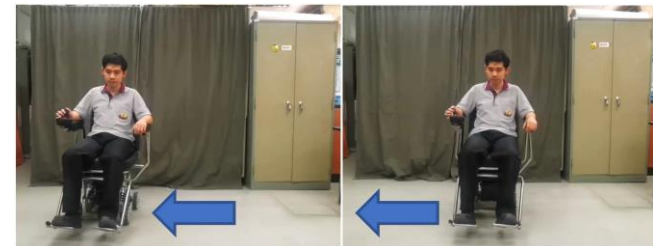
Fig. 27. Slide right testing of the electric wheelchair.
