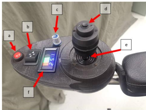
Fig. 3. The details of the joystick for the electric wheelchair.
