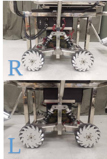
Fig. 9. An example of assembling the wheelbase of an electric wheelchair.
