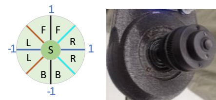
Fig. 12. Programming an analog joystick to allow control of a wheelchair without pressing the shift button.
