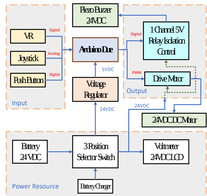
Fig. 1. A block diagram of the structure of the electric wheelchair.
