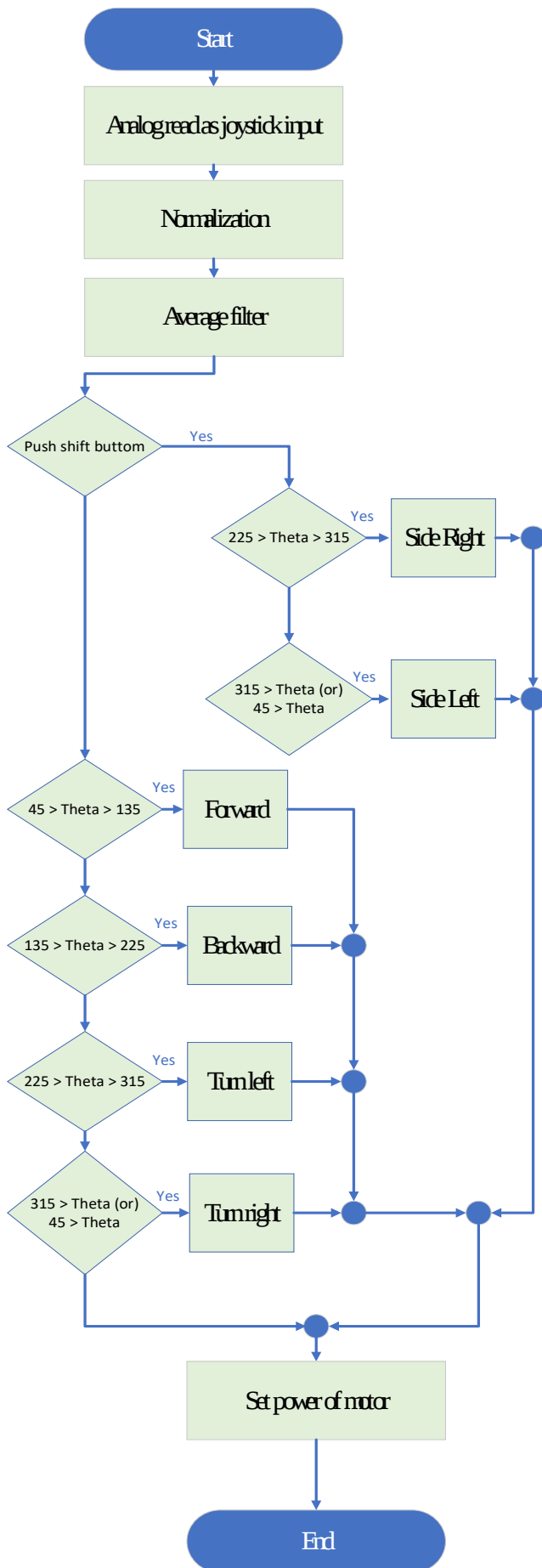
Fig. 11. System Flowchart.
