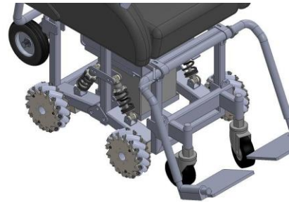
Fig. 8. The wheelbase of the electric wheelchair.
