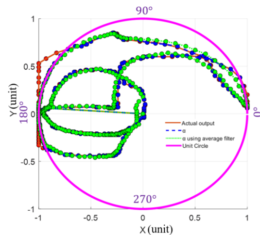
Fig. 20. The results of joystick movement.
