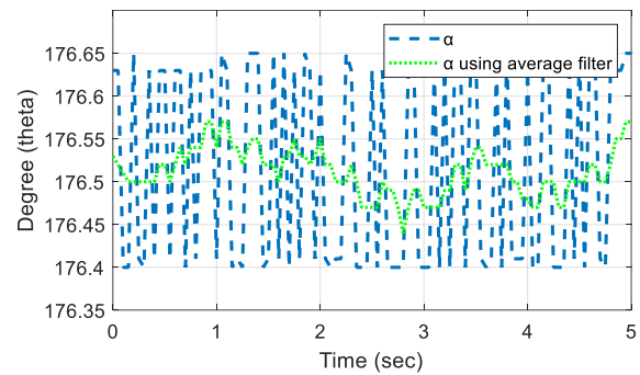
Fig. 19. The results of \theta in relation to joystick was held in place for 5 sec.
