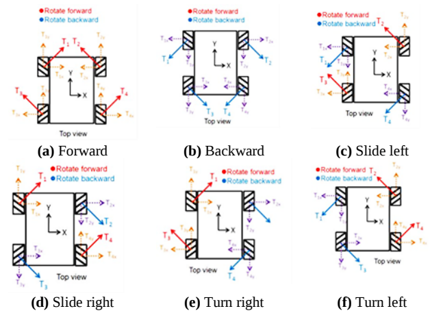
Fig. 16. The direction of movement of the mecanum wheel.
