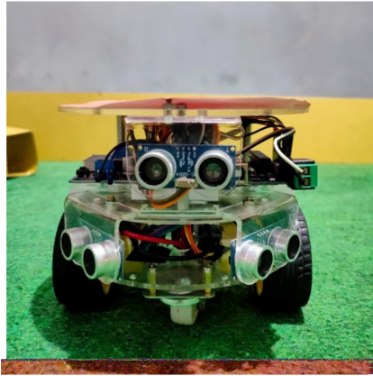
(b) Design of DDMR
