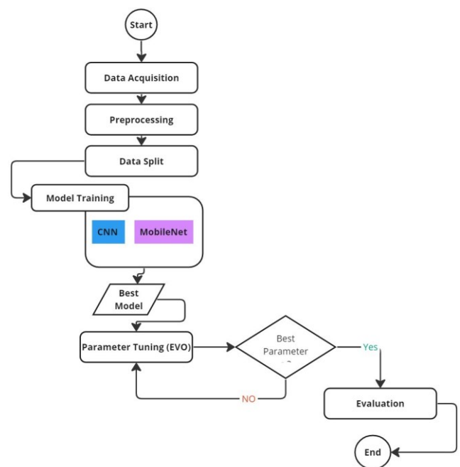
Fig. 1. General flowchart
