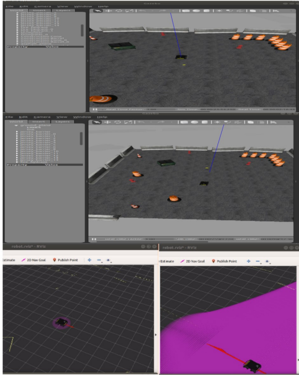
Fig. 20. Husky_robot in Gazebo and its map generation process based on SMC-NDO-NSO
