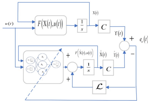
Fig. 3. Structure of a Neural State Observer (NSO)
