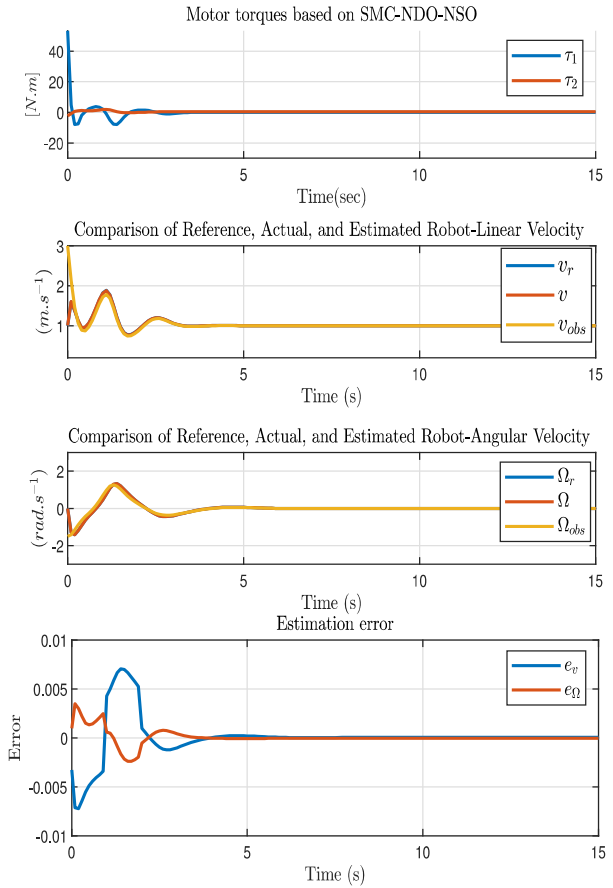
Fig. 6. Torque, Linear and angular velocities, and estimation error
