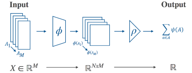
Fig. 7. Illustration of DeepSets concept
