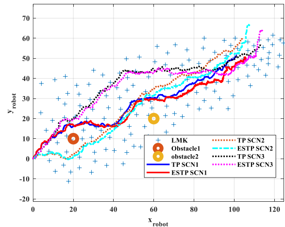
Fig. 10. Quadrotor motion with MCPP for scenario 2
