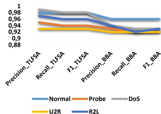
Fig. 4. Comparison of Precision, Recall, and F1-Score Between TLFSa and BBA Methods Across Network Traffic Classes (Normal, Probe, DoS, U2R, and R2L)
