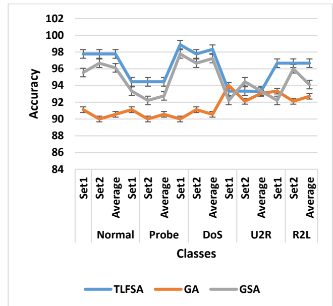
Fig. 3. The classification performance of the two subsets
