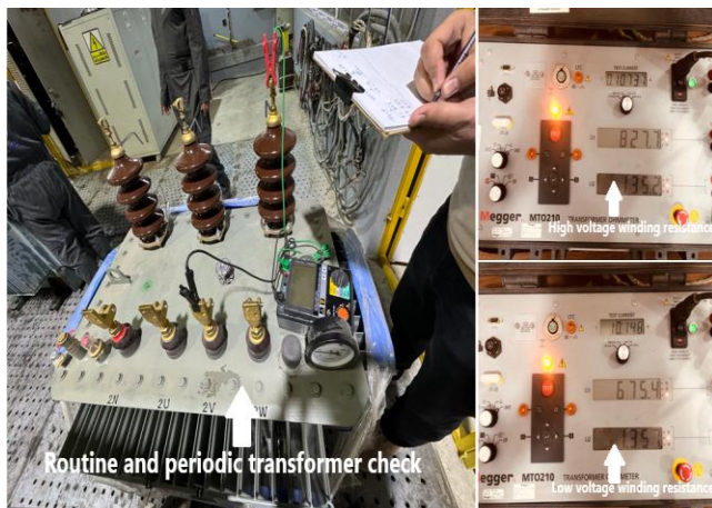
Fig. 3. Shows part of the tests conducted on a real model of a 1000 kVA transformer to determine the resistance values of the coils
