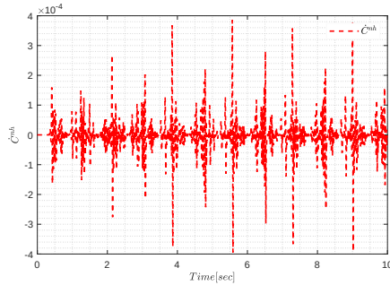
Fig. 8. Nonholonomic constraints violation \dot{C}^{nh}
