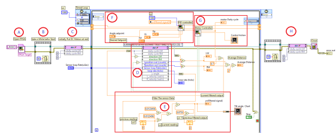
Fig. 37. The RT SBR PID Balancing Block Diagram vi
