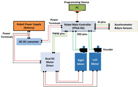
Fig. 31. System Hardware Block Diagram
