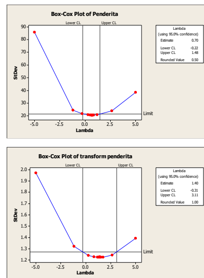
Fig. 3. Box-Cox test results for the number of people with schizophrenic disorders
