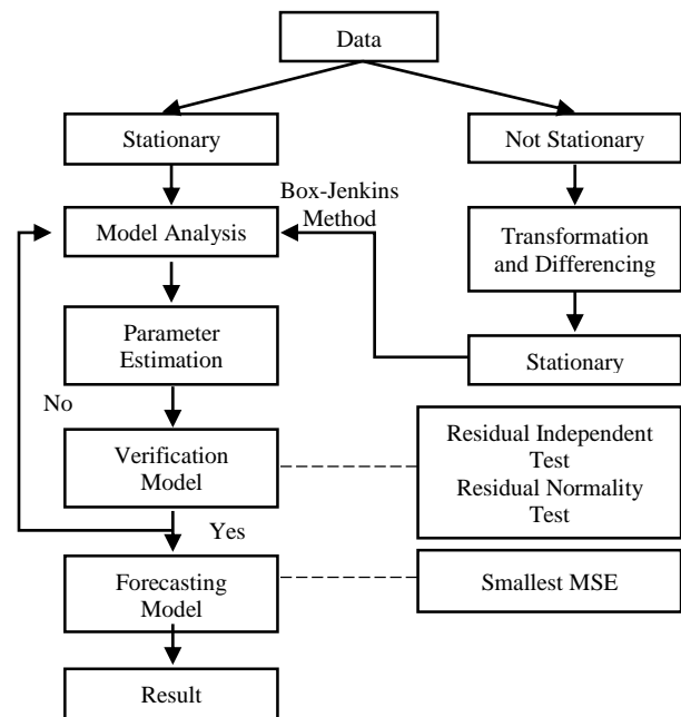
Fig. 1. Proposed Model
