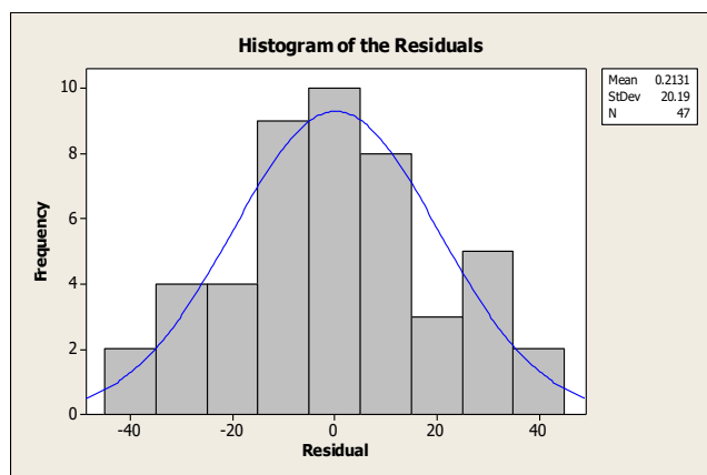
Fig. 9. ARIMA Residual Histogram (0,1,1)
