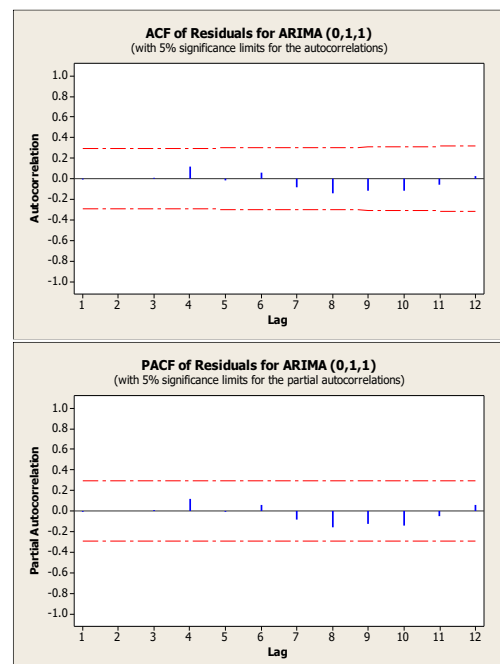
Fig. 8. Graphs of ACF and PACF Residual ARIMA (0,1,1)
