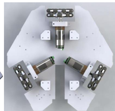
Fig. 7. (a) Chassis mechanical design; (b) chassis mechanical design perspective; (c) Omni wheel positioning design
