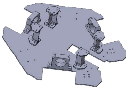
Fig. 7. (a) Chassis mechanical design; (b) chassis mechanical design perspective; (c) Omni wheel positioning design
