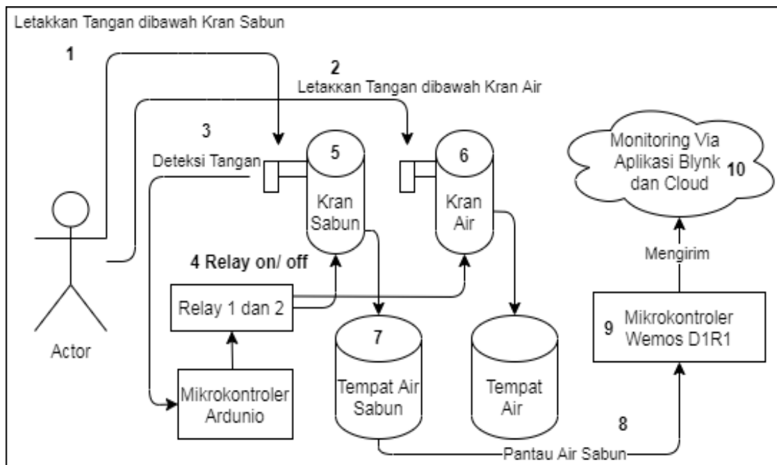
Gambar 3. Diagram Blok System
