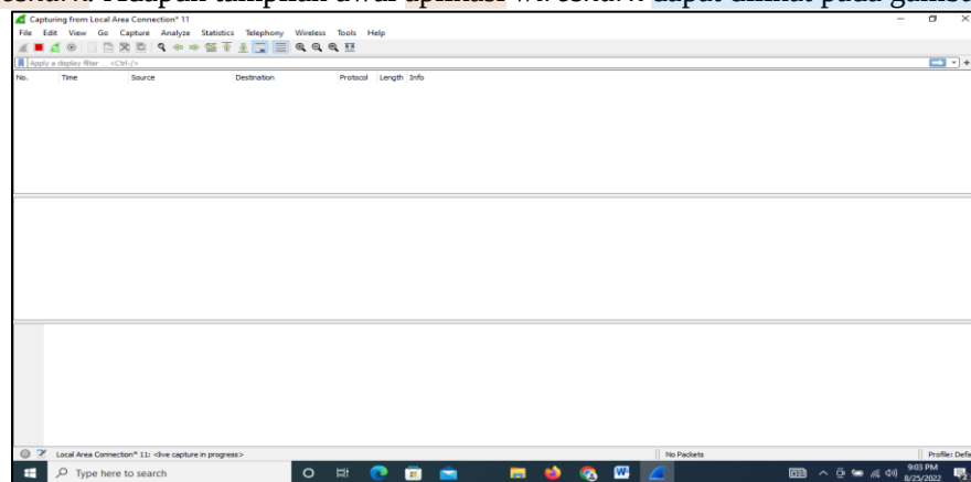
Gambar 12. Tampilan Wireshark
