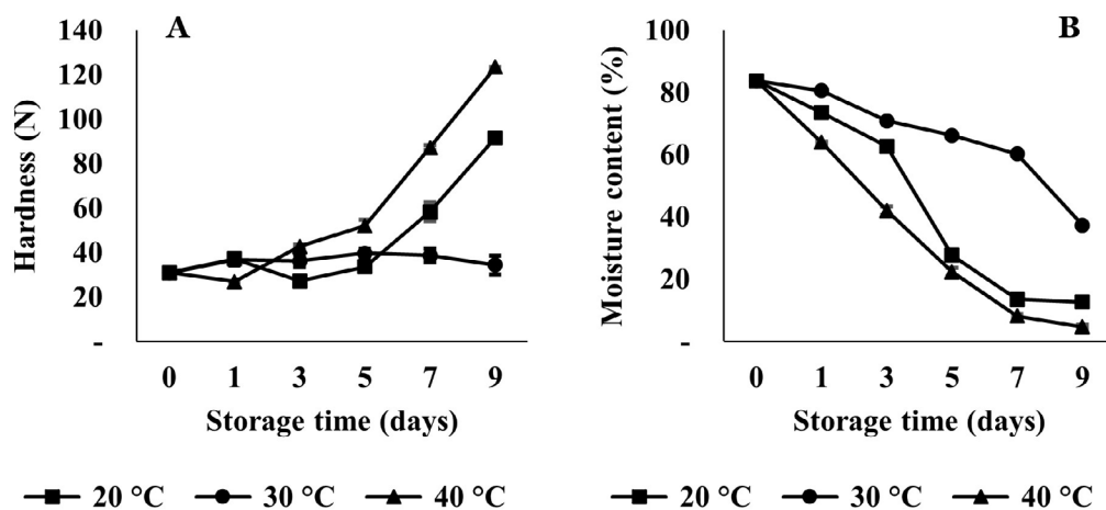
Figure 1. Changes in physical characteristics of CPH during storage. A) Pod husk hardness, N, Newton; B) moisture content.
