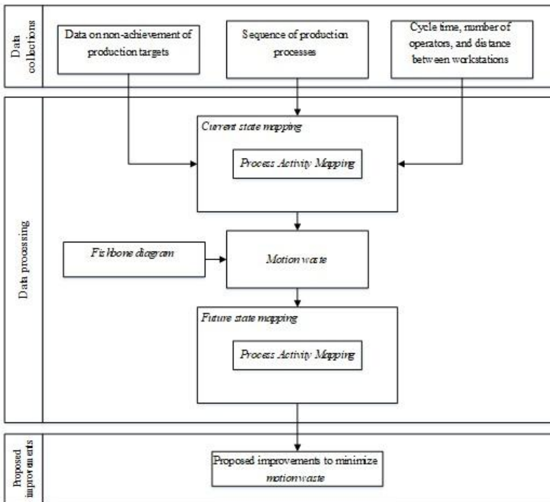
FIGURE 2. Research methodology
